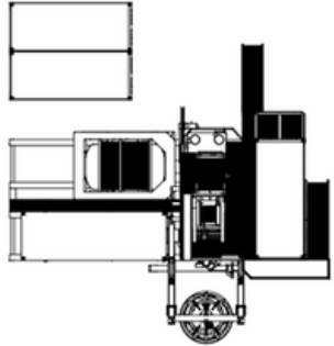
BOOM OUT TOP VIEW (A) SCALE 1:100
