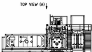
BOOM OUT FRONT VIEW SCALE 1:100
