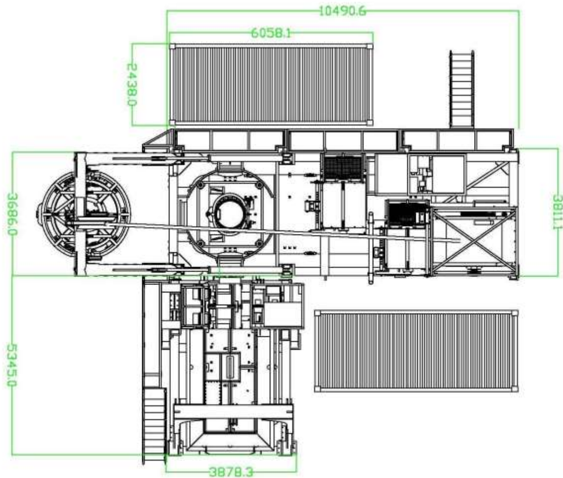
General Arrangement of DCN 9 man Saturation System
